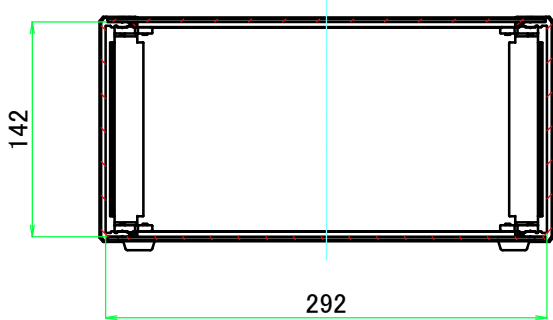
B-B (1:5)
