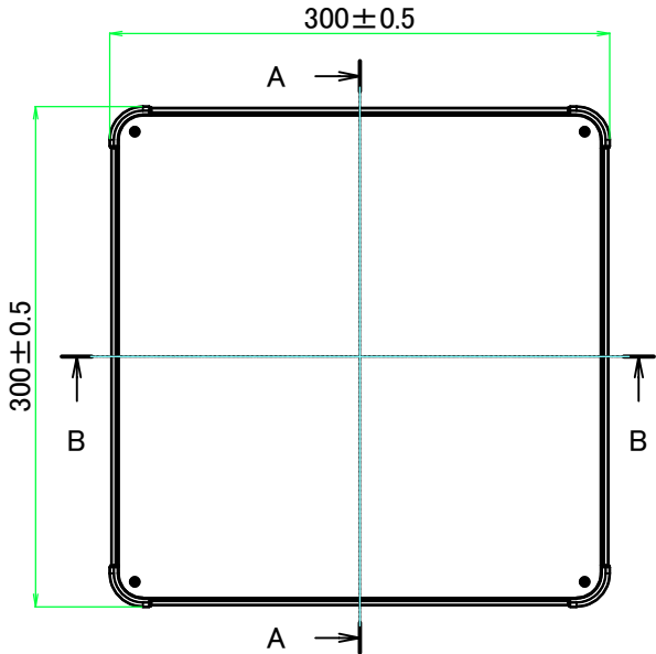
E view
