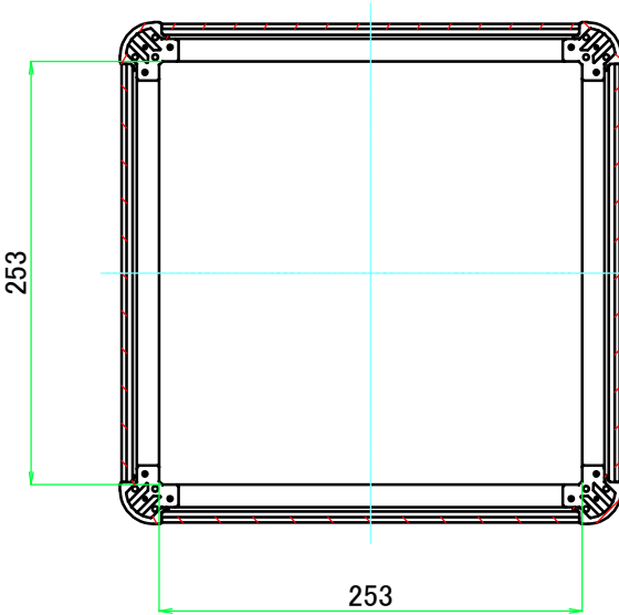
C-C (1:5)
