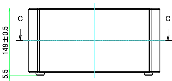
A view
